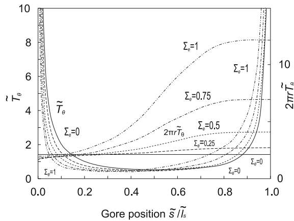
Fig. 2.11 Effect of \Sigma_c on the tension as a function of gore position. The right axis shows the total tensile force at a given gore position
