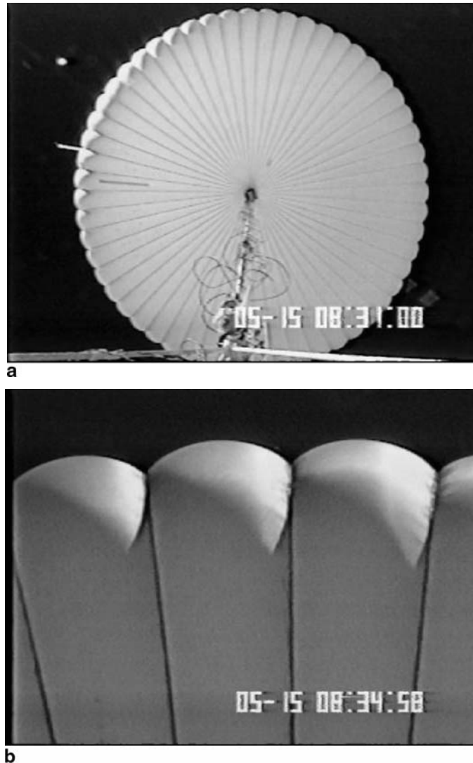
Fig. 2.20 Super-pressure balloon in flight. The bulges between the load tapes resulting from the 3D gore design concept are readily apparent: a Photograph of entire balloon; b Enlarged photograph
