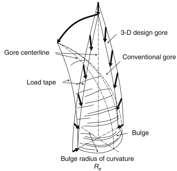
Fig. 2.18 Balloon-manufacturing method for the 3D gore design concept. A gore with a bulge is produced by attaching a gore that is larger than a conventional gore to the load tape by shortening (indicated by the thick arrows ). This process is similar to the 3D cutting procedures used for tailoring and dressmaking
