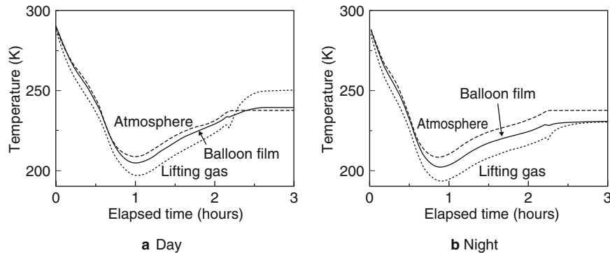
Fig. 2.33 Changes in atmospheric temperature, balloon film temperature, and lifting gas temperature. a and b correspond to day and night in Fig. 2.32, respectively: a Day; b Night
